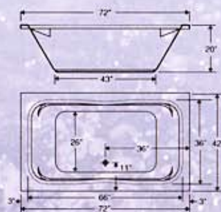
Model BRA-45 42"X72" Double Armrest Tub 82 Gallons
