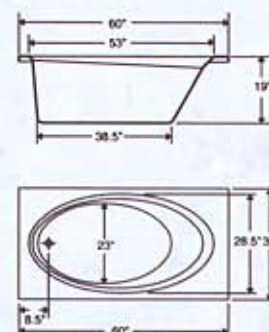
Model BR-19 32"X60" Oval Tub 54 Gallons
