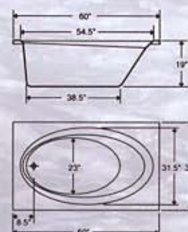
Model BR-24 36"X60" Oval Tub 55 Gallons
