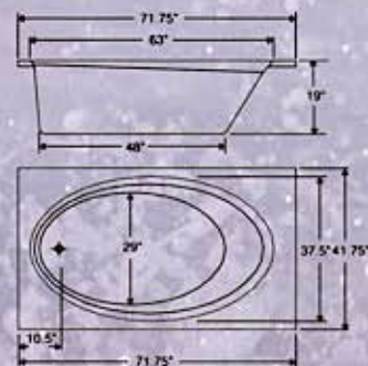
Model BR-32 42"X72" Oval Tub 79 Gallons
