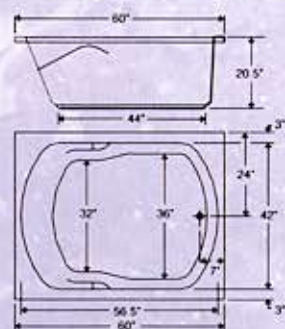
Model BRA-48 48"X60" Armrest Tub 75 Gallons
