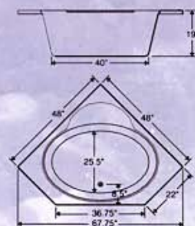
Model BR-49 48"X48" Corner Tub 70 Gallons
