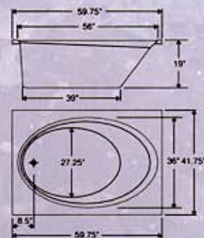
Model BR-33 42"X60" Oval Tub 65 Gallons
