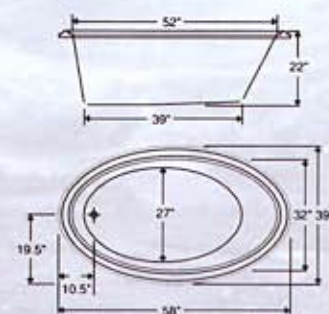
Model BR-20 39"X58" Oval Drop-In 65 Gallons
