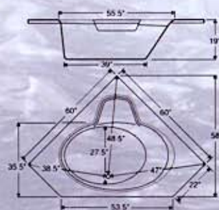
Model BR-41 60"X60" Corner Tub 75 Gallons
