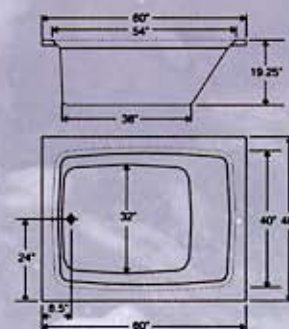
Model BR-35 48"X60" Tub 75 Gallons
