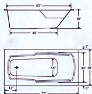
Model BRA-39 36"X72" Armrest Tub 70 Gallons
