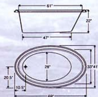
Model BR-40 41"X69", 6ft. Oval Drop-In 82Gallons
